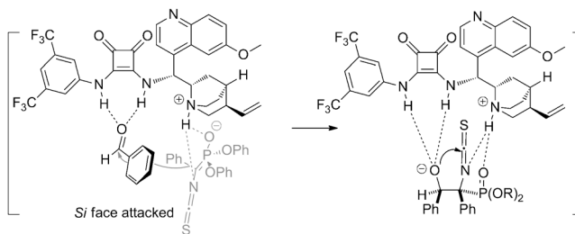
Scheme 2. Proposed transition states.
